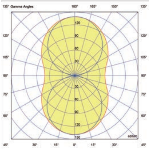
Archetto Space/2 strip LED
