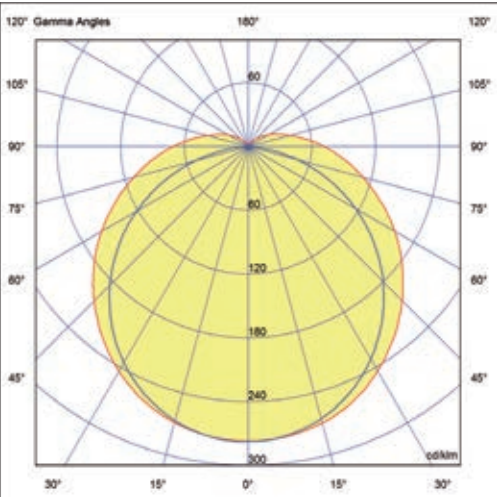
Archetto Space/1 strip LED
